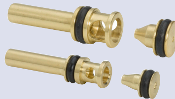
Top: Standard CM60 Min Series Cartridge 1.13" L x 0.31" dia. Bottom: Custom CM60 Min Series Cartridge 1.06" L x 0.24" dia.
