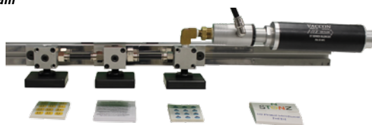
CDF 500H Custom Plenum - Pick & Place of multiple paper pads
